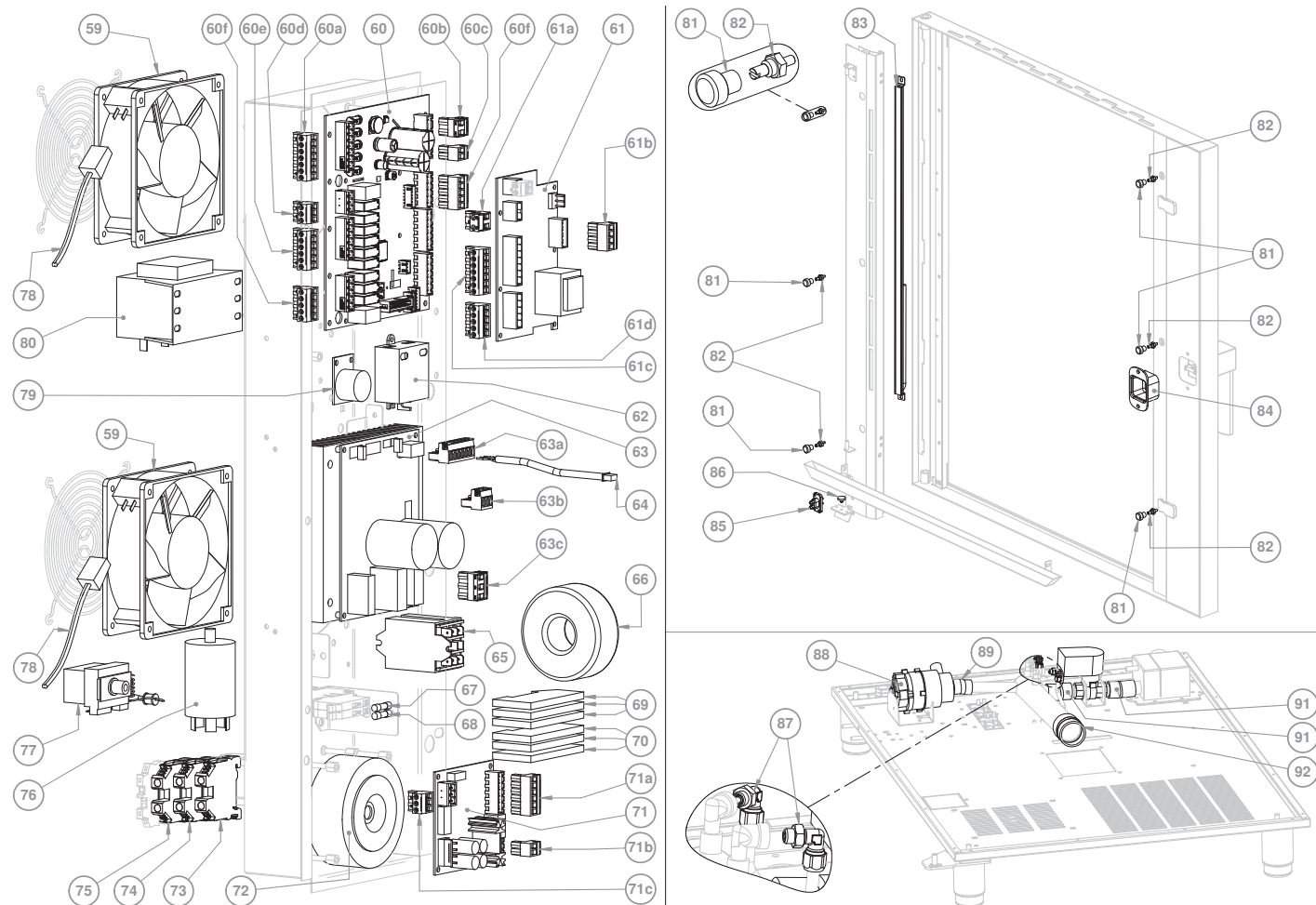
Exploded view 2/3
