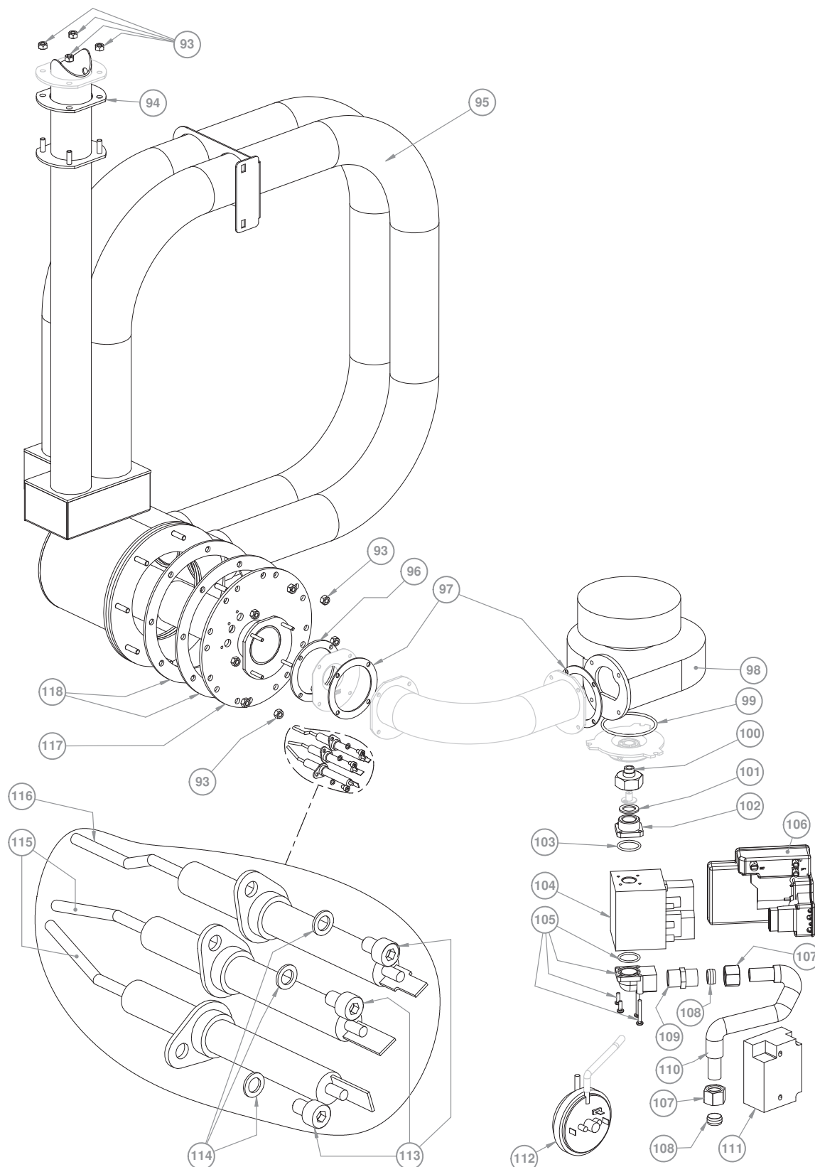
Exploded view 3/3
